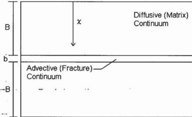
Figure 2.1. Parallel plate dual porosity conceptualization
