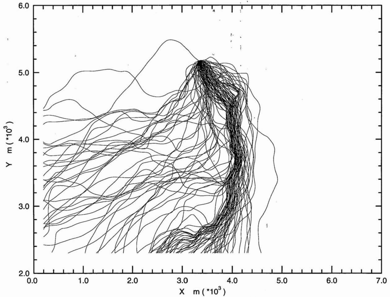
Figure 7.13 Replicate 1, full mining particle tracks
